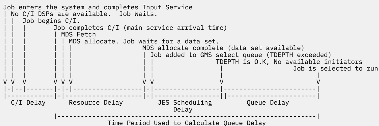
Figure 17: Overview of Pre-Execution Job Delays
